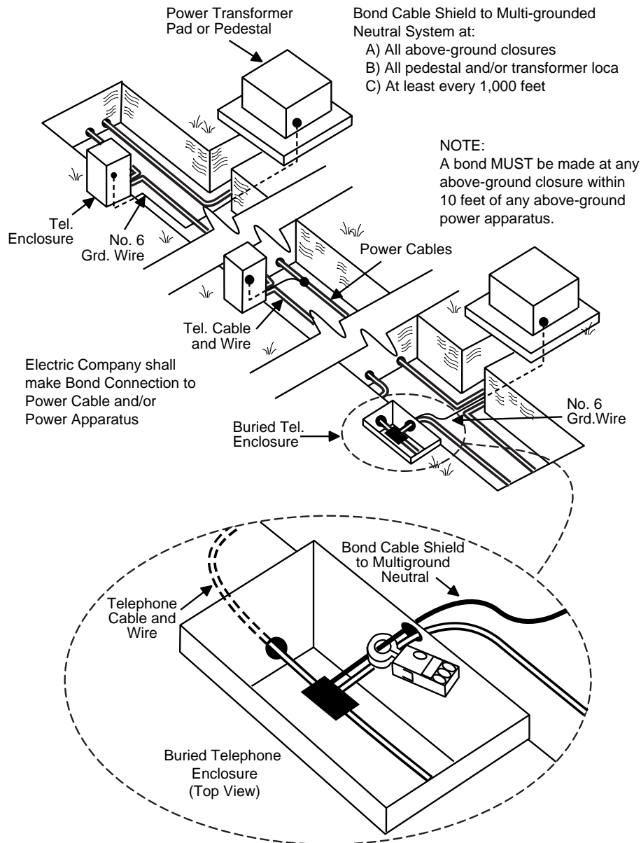
JOINT BURIED CONSTRUCTION – RANDOM SEPARATION
