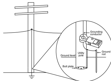
GROUNDING STRAND WITH NO OVERHEAD POWER
