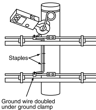
GROUNDING STRAND WITH NO OVERHEAD POWER
